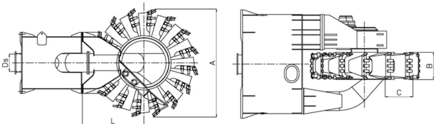
structural drawing
