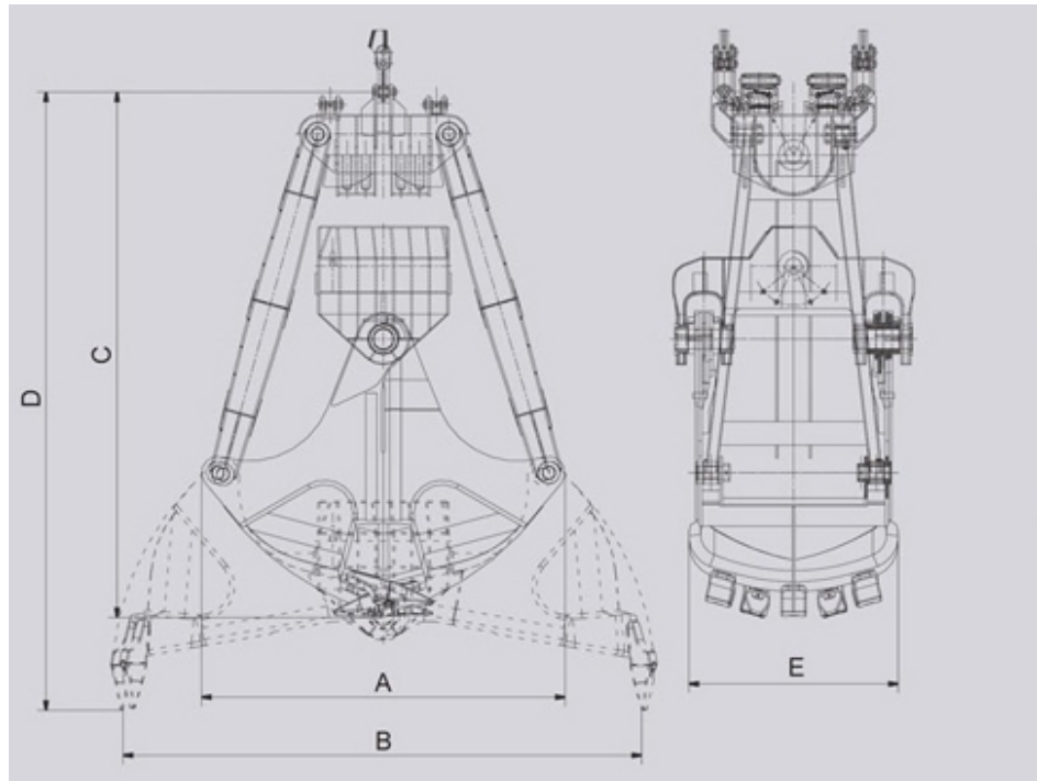
Four rope dredging grab Drawing
