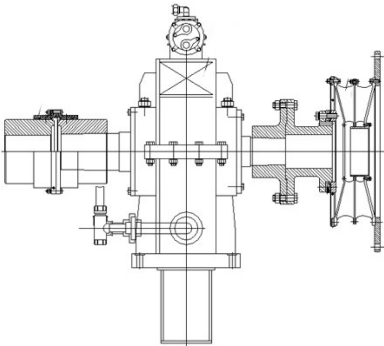
structural drawing
