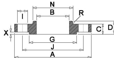
Slip-on flange
