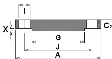
Blind flange
