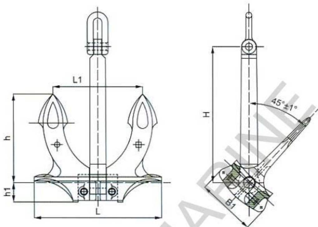
TYPE A MARINE HALL ANCHOR
