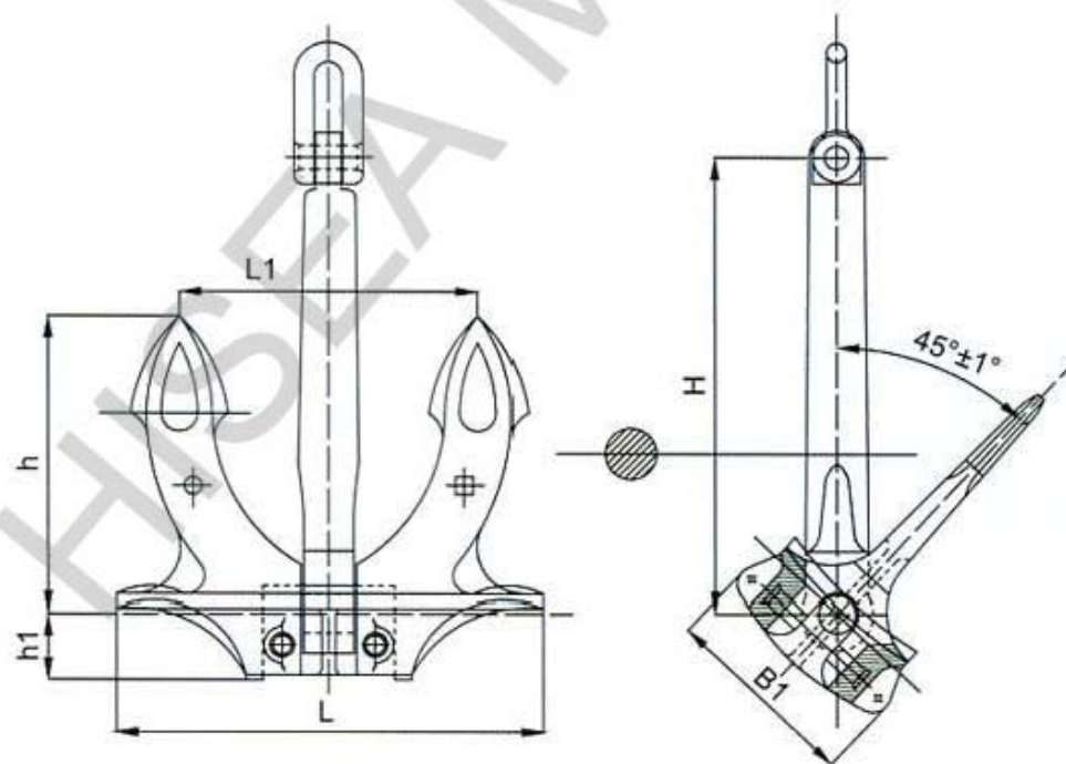
TYPE B MARINE HALL ANCHOR
