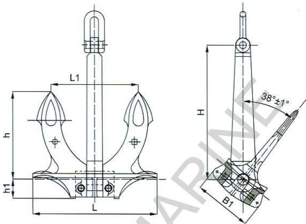
TYPE C MARINE HALL ANCHOR
