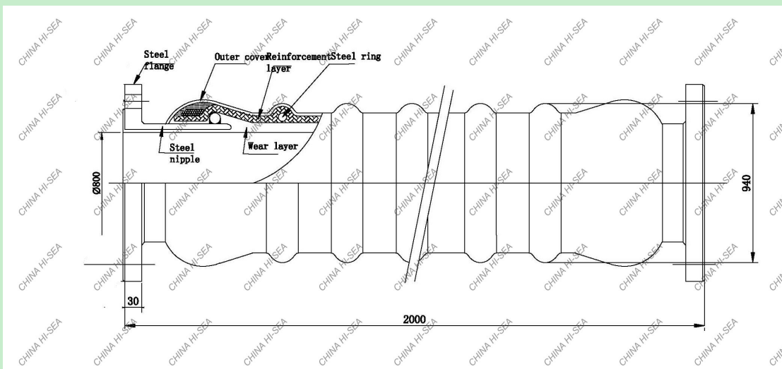
DN800 dredging discharge hose drawing
