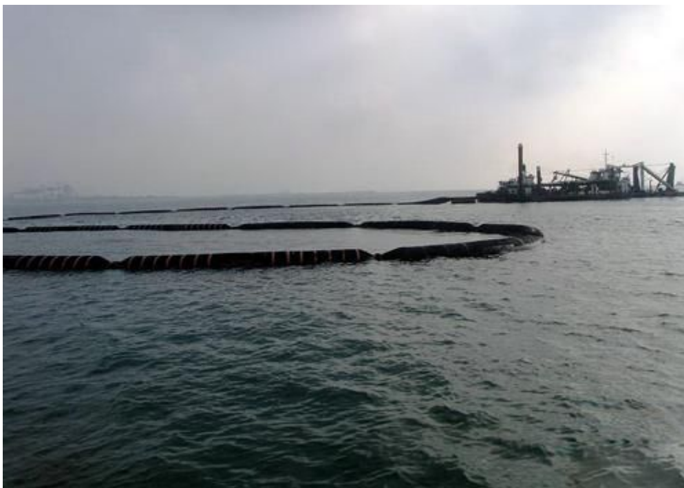
Floating hose in overseas construction site
